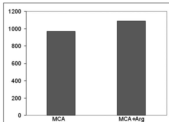
Figure 2. The effect of L-arginine supplementation on methylcholanthrene induced tumor growth.
