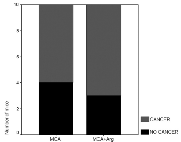
Figure 1. The effect of L-arginine supplementation on methylcholanthrene induced carcinogenesis.
